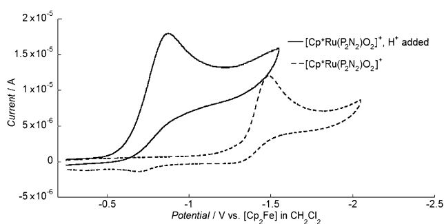
Figure 3. Cyclic voltammograms of [\text{Cp}^*\text{Ru}(\text{P}_2\text{N}_2)(\text{O}_2)][\text{PF}_6] (1.2 mM) (gray, dashed line) and [\text{Cp}^*\text{Ru}(\text{P}_2\text{N}_2)(\text{O}_2)][\text{PF}_6] with HOTf added (black, solid line) in \text{CH}_2\text{Cl}_2 , 0.1 M n\text{Bu}_4\text{N}^+[\text{PF}_6]^- , scan rate 0.1 \text{Vs}^{-1} .
