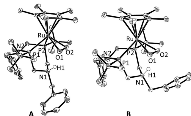
Figure 2. ORTEPs of two different structures of [Cp^*Ru(P_2N_2H)(O_2)][PF_6]_2 : A ( 1/4 H_2O ), left, and B ( 1/2 MeOH ), right, with thermal ellipsoids shown at 50% probability. For clarity, the solvent molecules, counterions, and hydrogen atoms except for the hydrogen-bonding H1, have been omitted.
