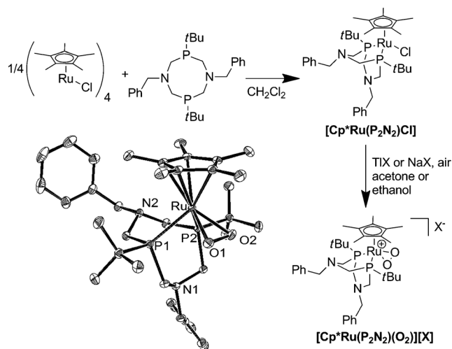
Figure 1. Synthesis of [Cp^*Ru(P_2N_2)(O_2)][X] and ORTEP diagram of the cation in [Cp^*Ru(P_2N_2)(O_2)][BPh_4] . Thermal ellipsoids are shown at 50% probability. For clarity, hydrogen atoms have been omitted.
